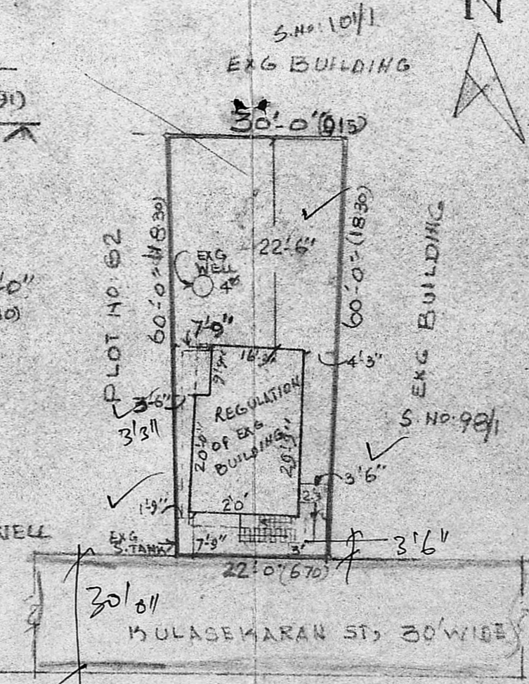
SITE PLAN SCALE 1" = 24'-0"
